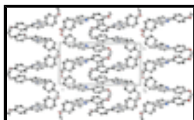
Fig. 2. The crystal packing diagram of the title compound, viewed down the a axis (Hydrogen atoms have been omitted for clarity).
